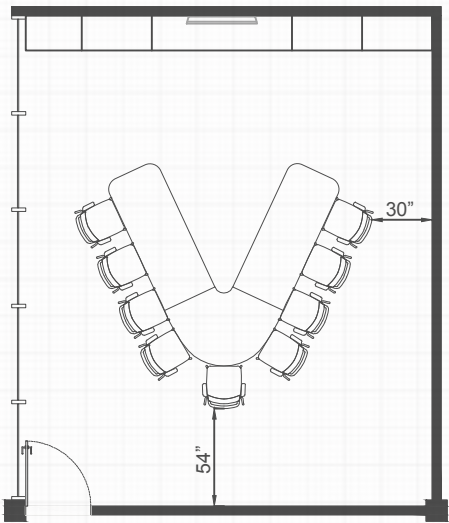
ALP9648SH with multi-purpose seating
