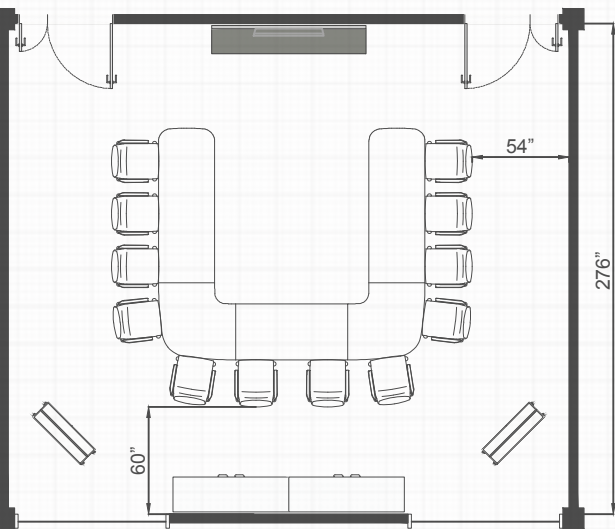
ALP138134UR with conference seating
