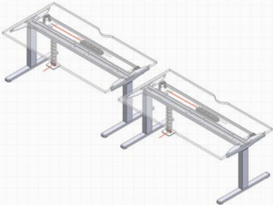
Typical I-leg desk wiring layout.
