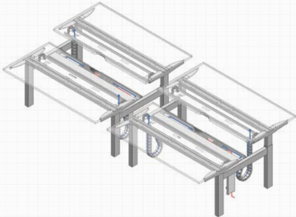
Typical H-leg desk wiring layout.
