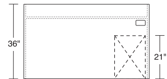
1524 Pedestal (21" deep)
