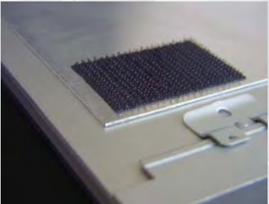
VELCRO (V) Industrial strength velcro hook applied to module back... excellent solution for panels with a weave fabric.
