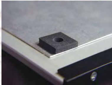
SCREW (S) Ideal for larger signs. Equipped with hard rubber spacer-grommet around screw holes on back side protects the wall and provides equal pressure around screws. Screw heads are hidden behind the message tiles.
