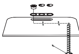
Netbox Point Single + Alu Cover incl. cable management
