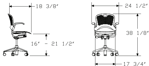
FLEXNET Seat
