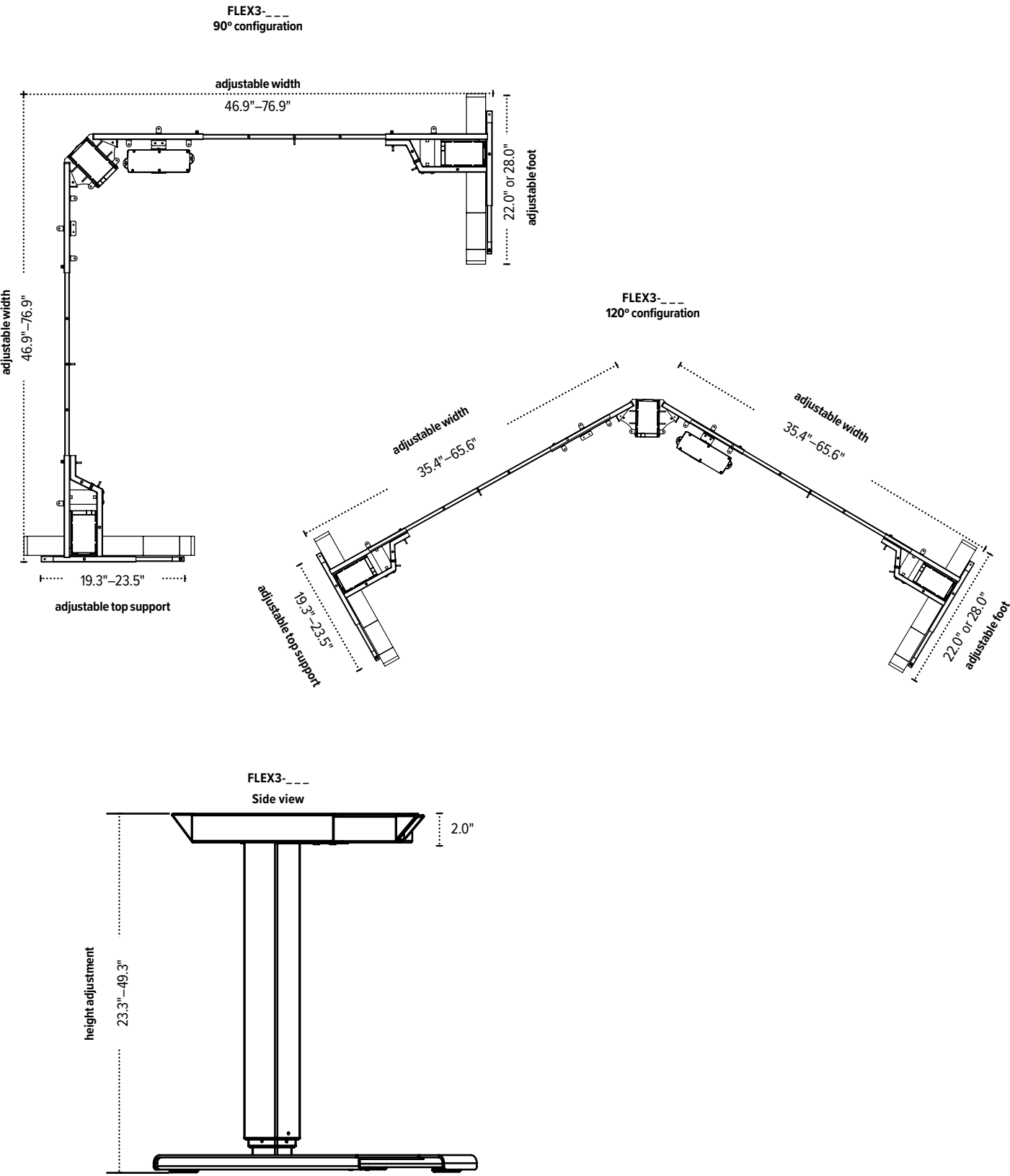
The base dimensions as shown are actual.
