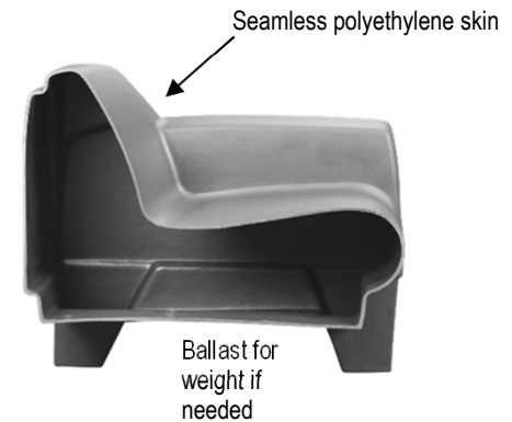
Cross-section of rotationally molded plastic lounge chair
