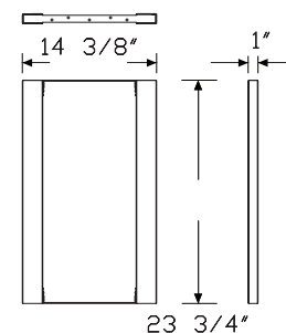
Open stanchion
