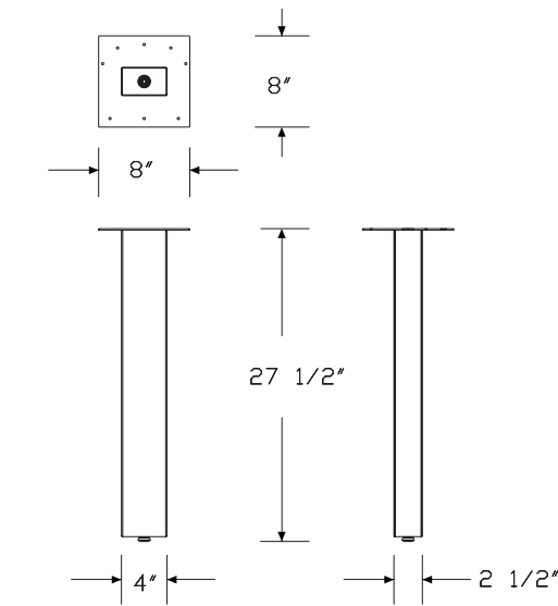
Square Leg
