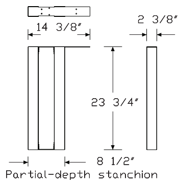
Partial-depth stanchion
