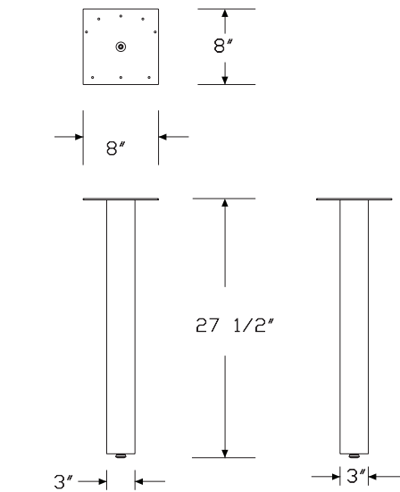
Round Leg
