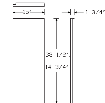
Solid stanchion
