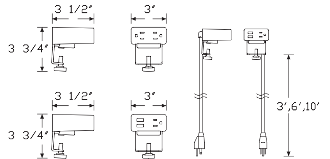
Surface Clamp
