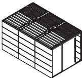
OB1AIR27 Rectangle with Opening Roof External: 14'5"D x 9'2"W x 8'4"H Internal: 14'1"D x 8'7"W x 7'H
