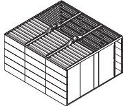
OB1AIR29 Square 3x3 with Opening Roof External: 14'4"D x 13'4"W x 8'4"H Internal: 14'1"D x 13'W x 7'H
