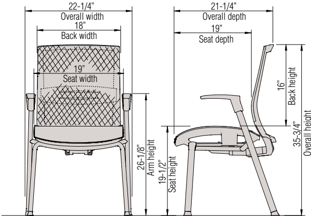
Guest Chair
