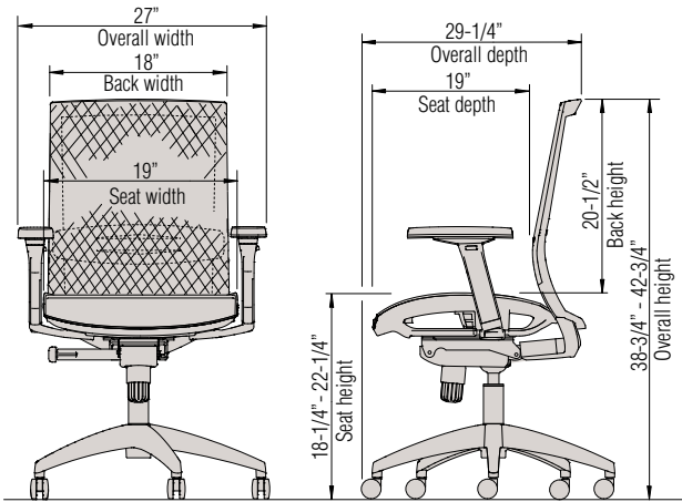
Task Chair
