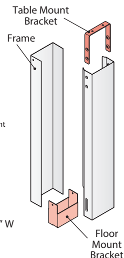
Cable Column: Exploded View
