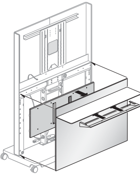
EWVX-SB7P-N1 Easel Tile with (1) Shelf (Standing Ht. 52"-55" Monitor)
