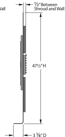
Side View – 3 1/8" deep radius edge shelf
