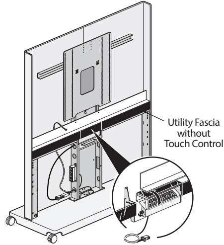
Mobile Monitor Easel – For Non-Switching Interface Module
