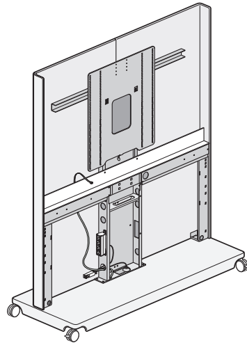
Mobile Monitor Easel – No Interface Module
