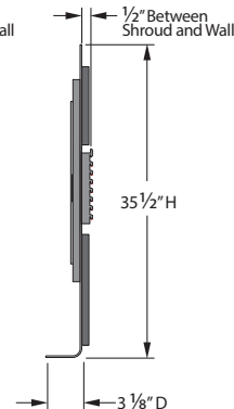
Side View – 3 1/8" deep radius edge shelf
