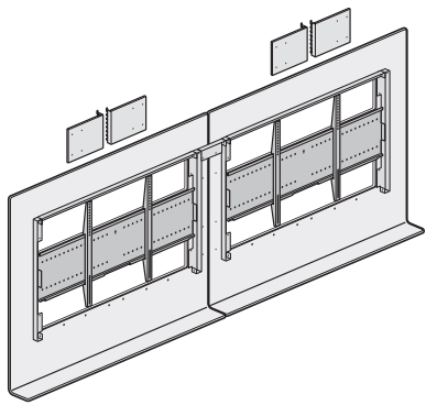
Dual Monitor With Shroud 3 1/8" Deep Radius Edge Shelf EWVE-D_SS-PP
