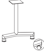
Metal Cantilever T Base 23" Span • fixed base style • fixed base with casters* • tilt base style • tilt base with casters* ship as a set of 2 bases with cables and lever
