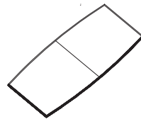
boat 144" x 48" 3 bases seats 12 120" x 48" 2 bases seats 8 96" x 48" 2 bases seats 8 72" x 36" 2 bases seats 6
