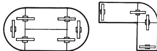
Figure 9 - 90° Leg Connections
