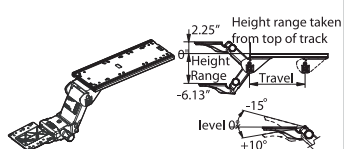
Lift-N-Lock Sit-Stand Mechanism
