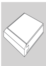
Veneer-Facet; solid wood T-edge on 1-1/8" particleboard (FA)
