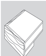
Laminate; 3/8" x 1-3/4" wood band edge; square corner; corner joint is not mitered (36S)
