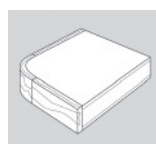
Laminate; 3/8" x 1-1/4" wood band edge; radius corner (34R)
