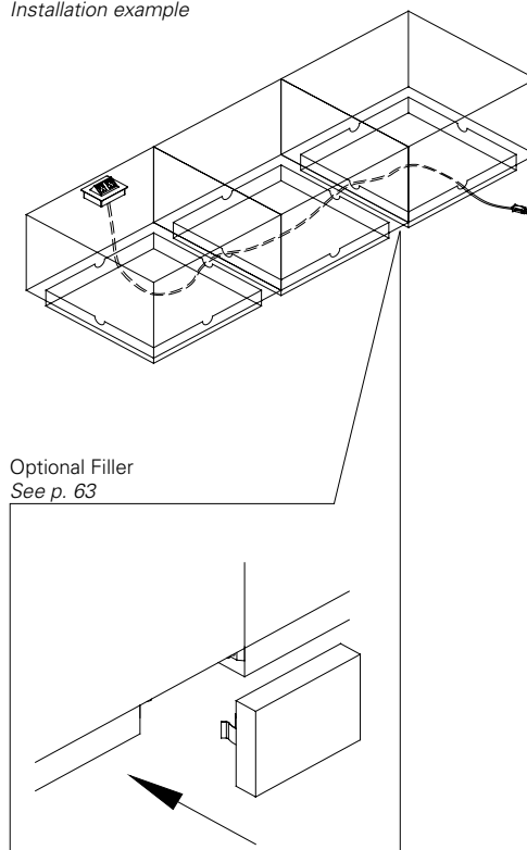
Installation example
