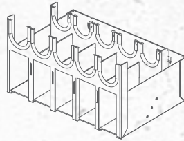
TCP-5S-XXX Pistol Rest; 5-Cap; w/Magazine Storage
