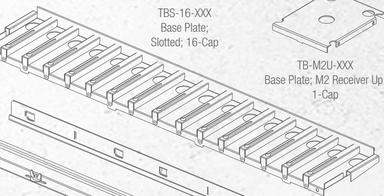
TCX-20-XXX Bin Bar for Plastic Bins; 20W
