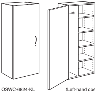
OSWC-6824-KL (Left-hand with lock, closed view)
