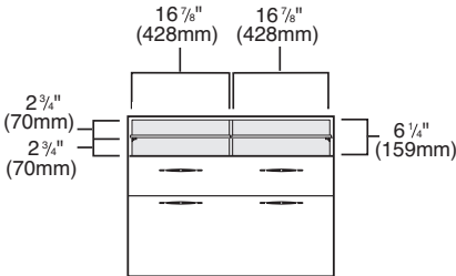
Lateral storage interior shelf dimensions
