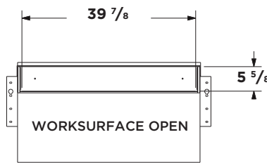
42" WORKSURFACE
