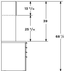
OVERHEAD ZONE = 39H TACK ZONE = 26H
