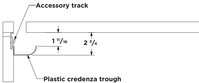
Side View - shown with accessory mounted into accessory track
