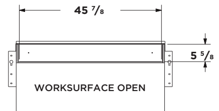
48" WORKSURFACE
