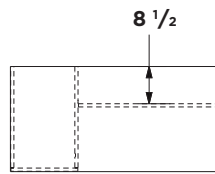
WALL ACCESS PANEL CLOSED (TOP VIEW)
