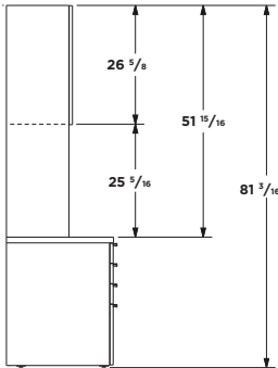
OVERHEAD ZONE = 52H TACK ZONE = 26H
