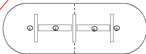
Two-Piece Conference Table with 2-3/8" Panel Legs and Wire Management Stretcher Trough
